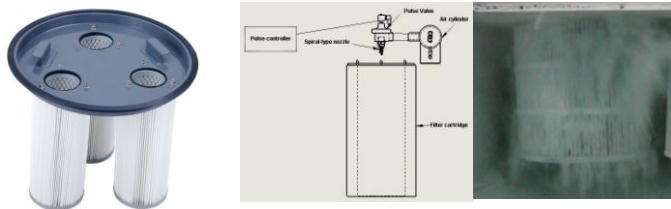
The principle of auto air pulse jet cleaning
