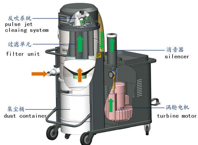
Structure Diagram
